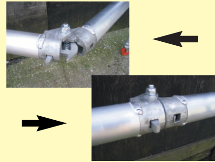
CENTRAL AUTOMATIC LOCKING DEVICE
