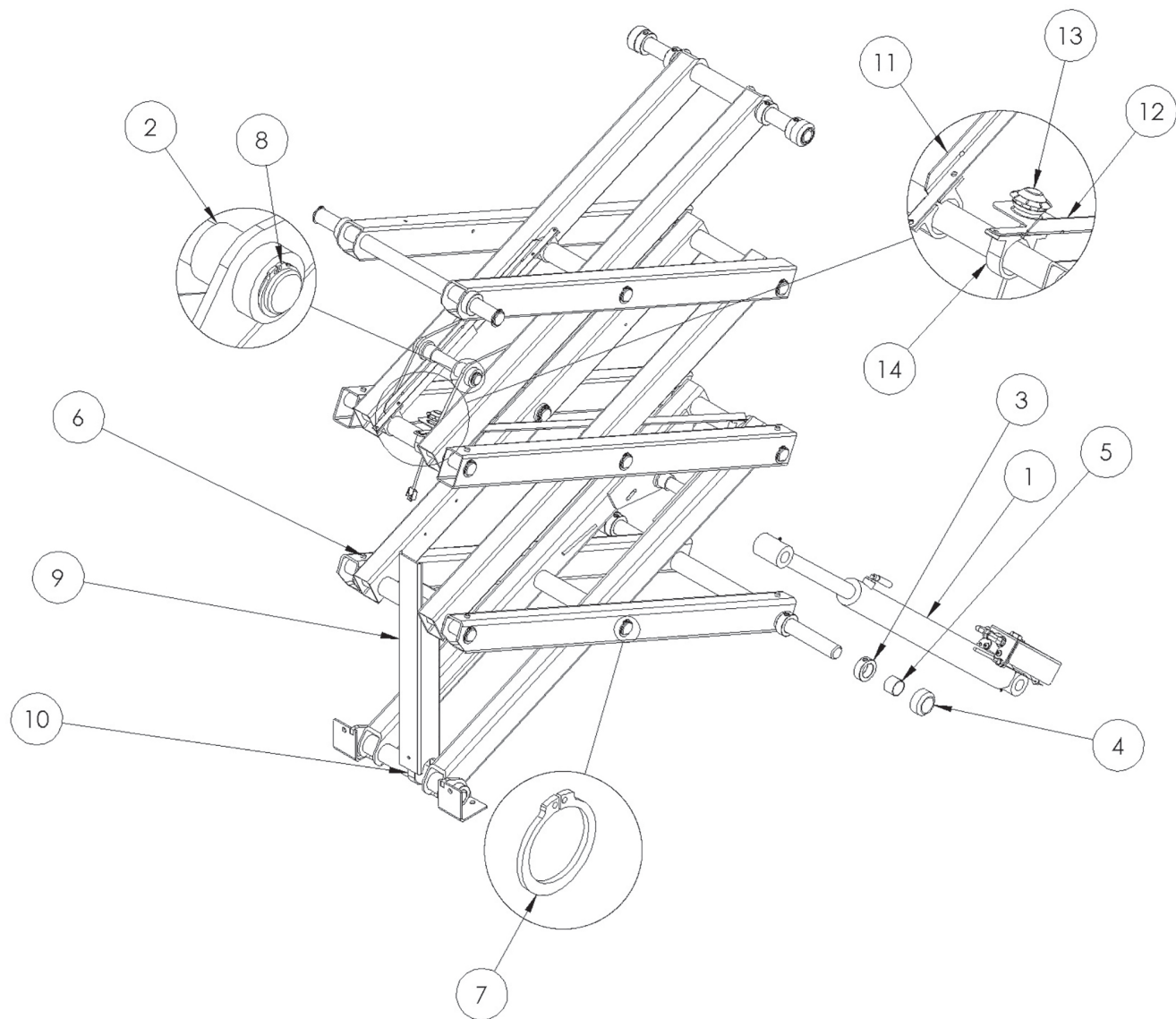
FIGURE 13: Scissor Parts
