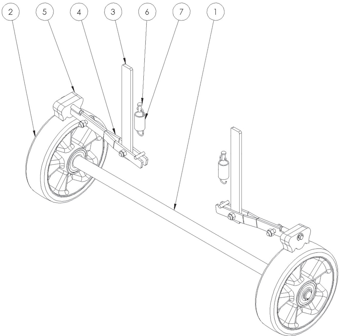
FIGURE 2: Brake Subparts
