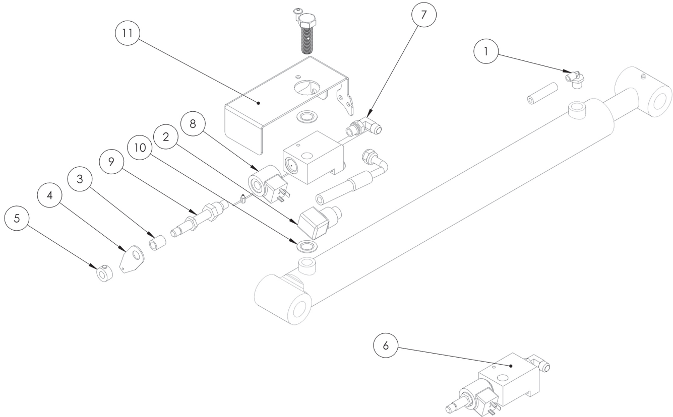
FIGURE 14: Cylinder Subparts
