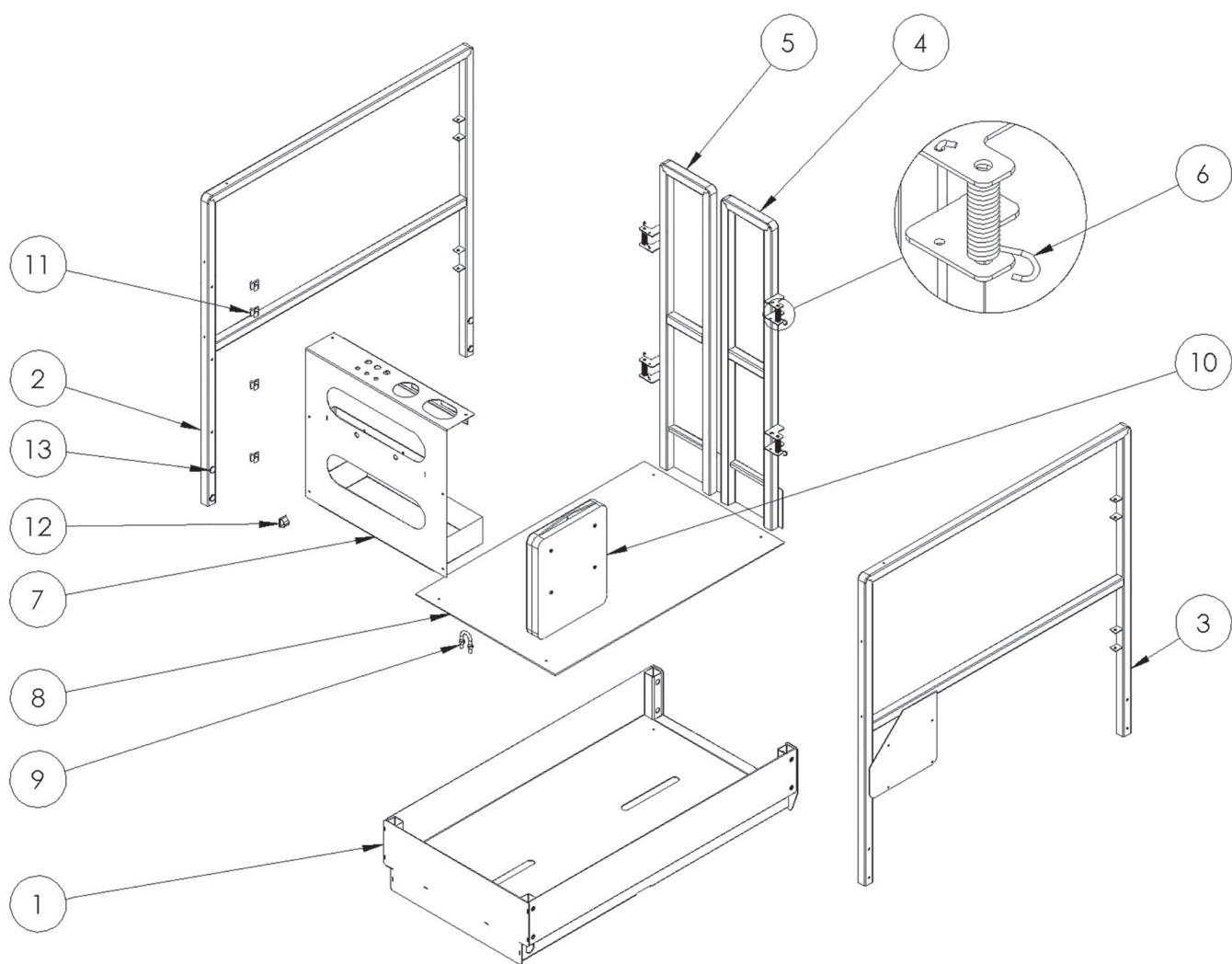
FIGURE 15: Platform and Rails
