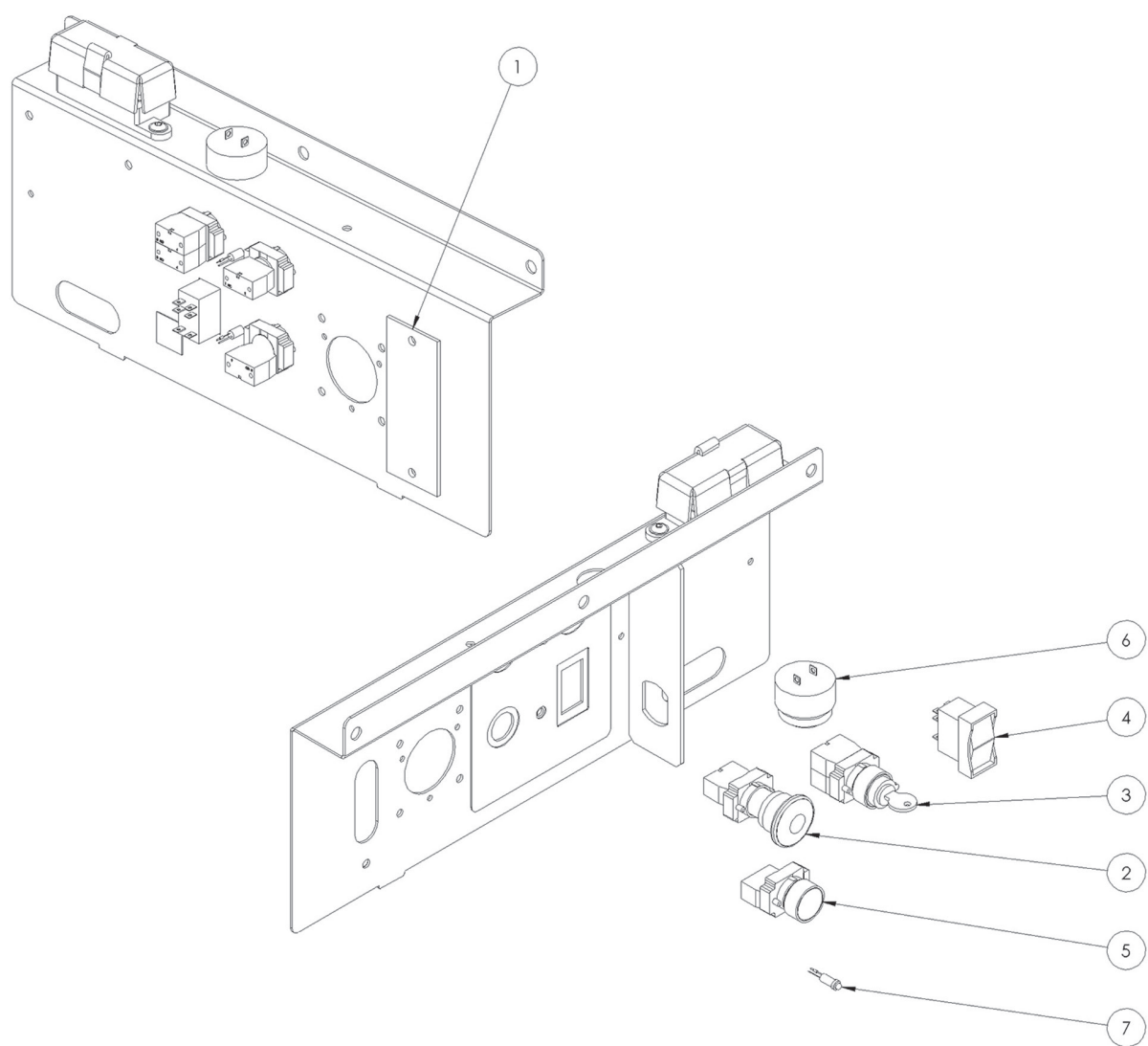
FIGURE 9: Ground Control Parts
