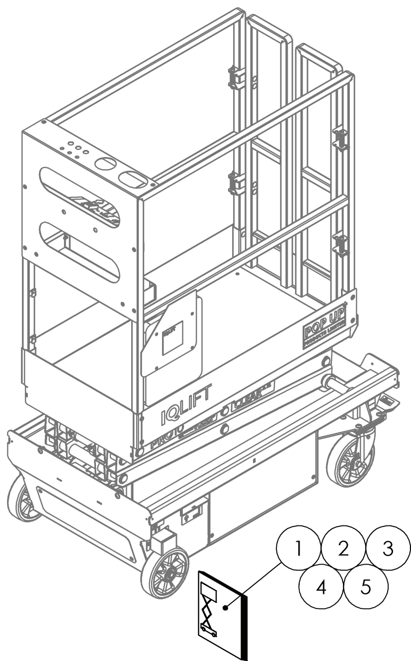
FIGURE 17: Options and Miscellaneous
