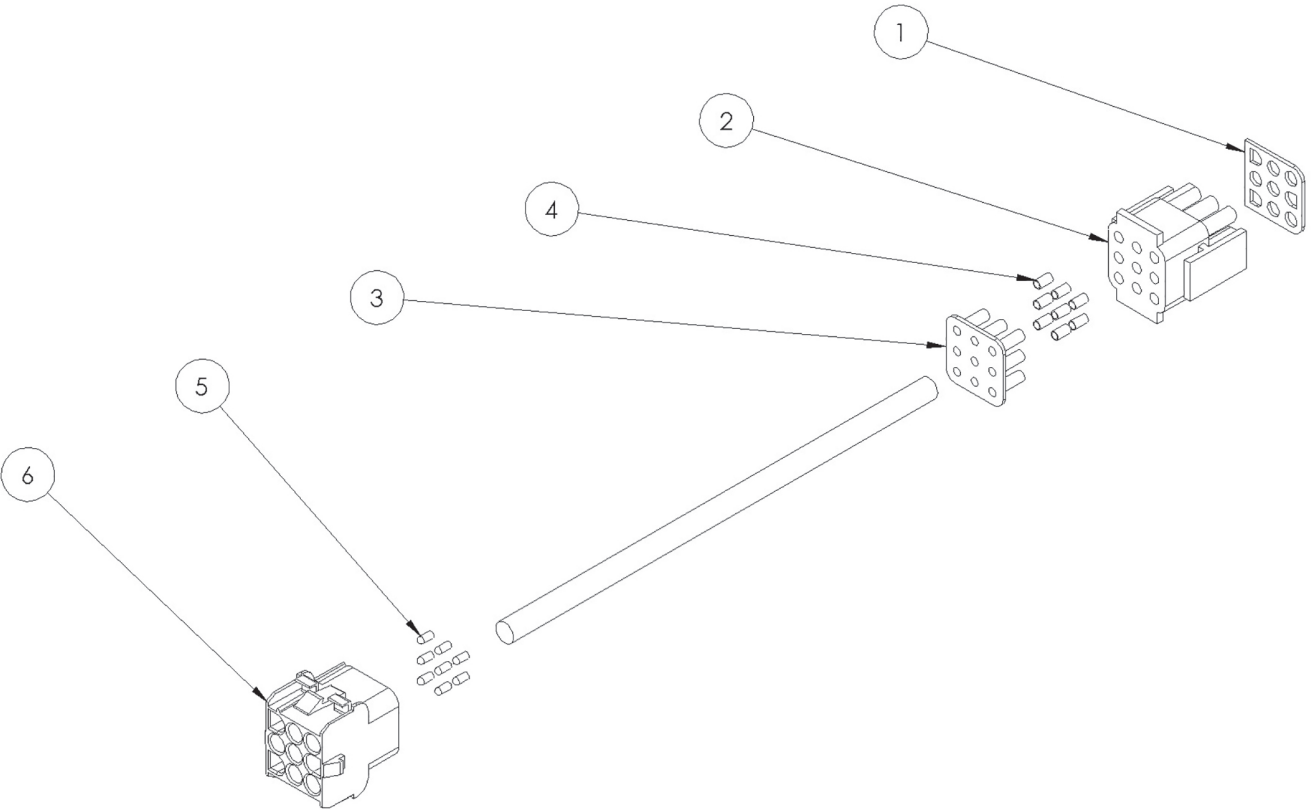
FIGURE 7: Main Cable Subparts
