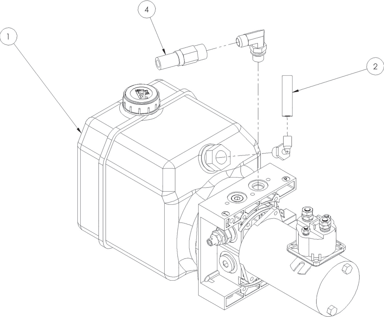
FIGURE 3: Pump Parts
