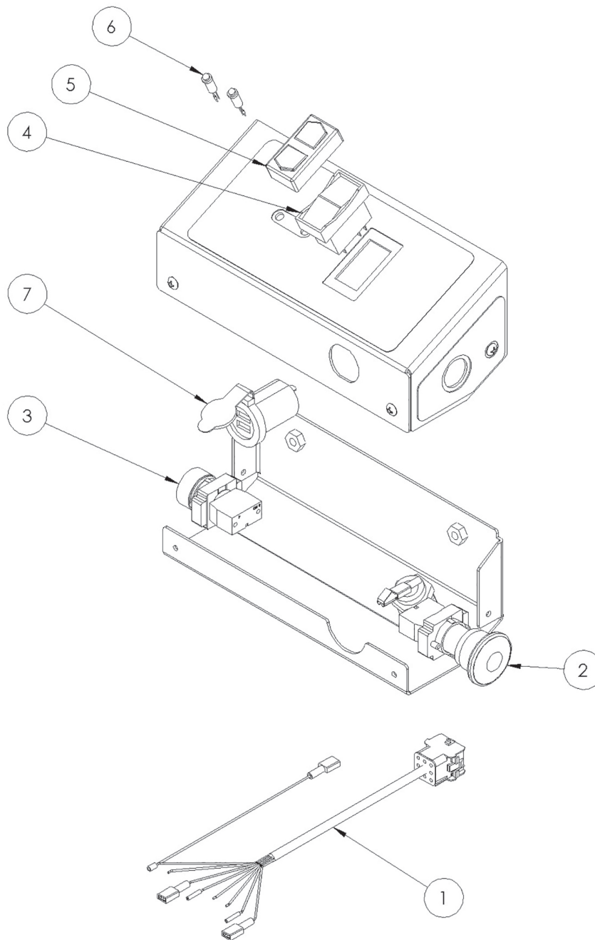
FIGURE 8: Platform Control Parts
