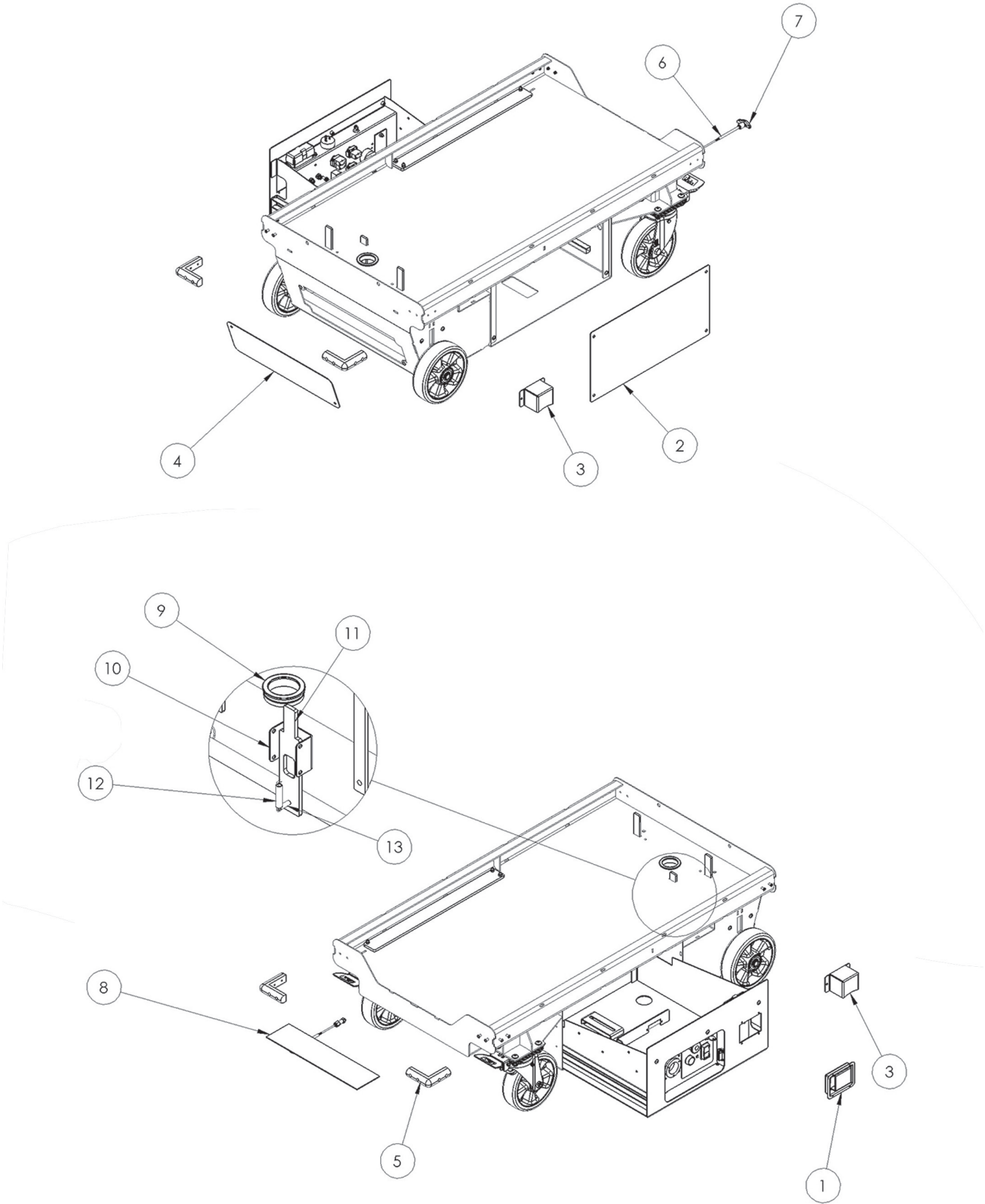
FIGURE 5: Miscellaneous Parts
